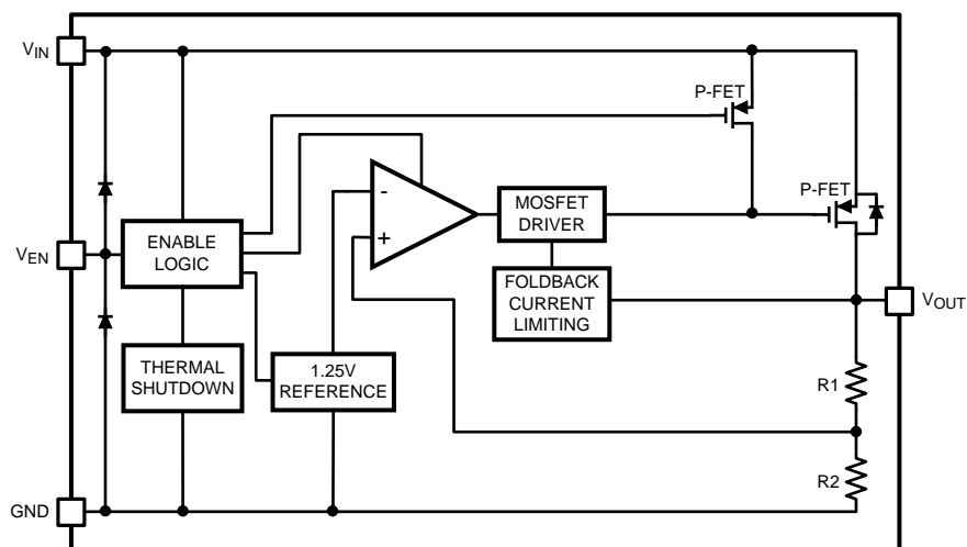
Figure 8. LP38693 Functional Diagram (SOT-223)
