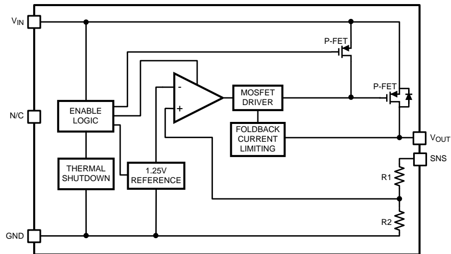
Figure 5. LP38691 Functional Diagram (LLP)
