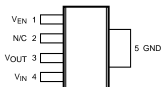
Figure 2. SOT-223, Top View LP38693MP-X.X
