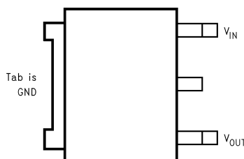
Figure 1. TO-252, Top View LP38691DT-X.X
