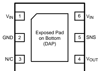
Figure 3. 6-Lead LLP, Top View LP38691SD-X.X
