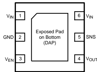
Figure 4. 6-Lead LLP, Top View LP38693SD-X.X
