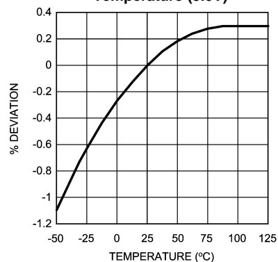
V_{OUT} vs Temperature (5.0V)
