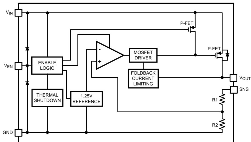
Figure 7. LP38693 Functional Diagram (LLP)
