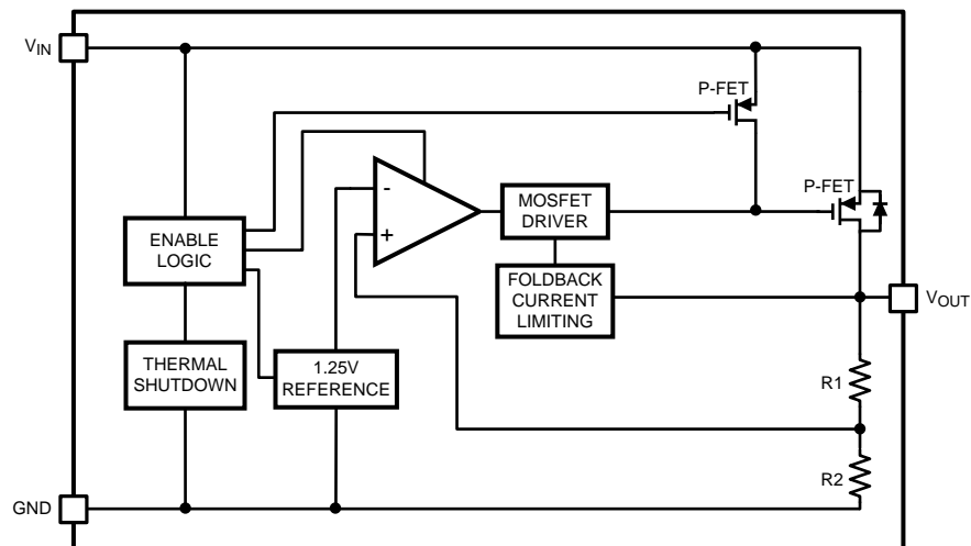
Figure 6. LP38691 Functional Diagram (TO-252)
