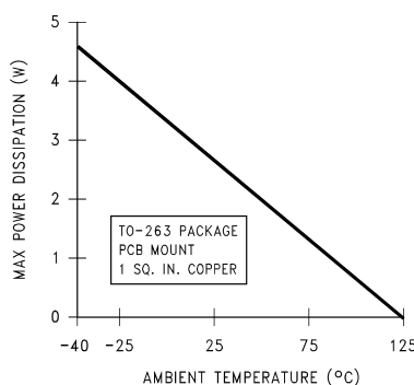
Figure 22. Maximum power dissipation vs ambient temperature for DDPAK/TO-263 package
