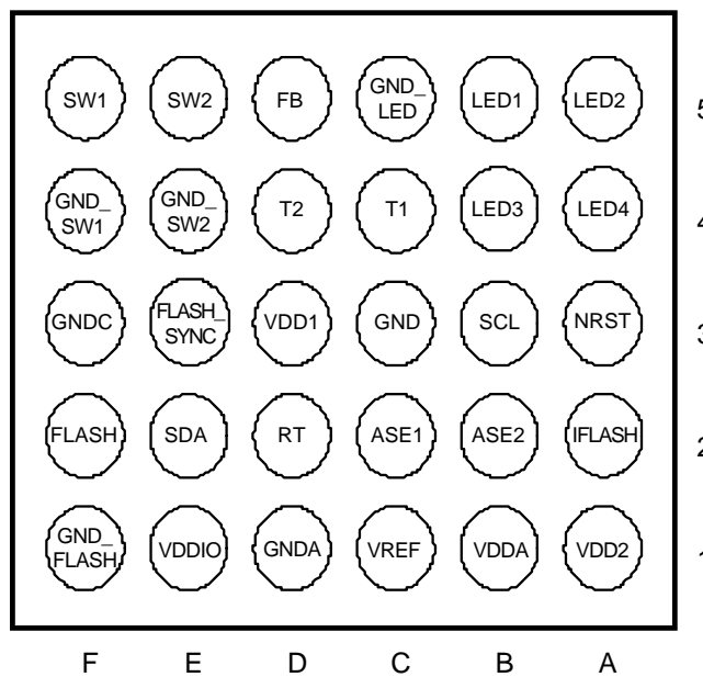
Figure 2. Bottom View
