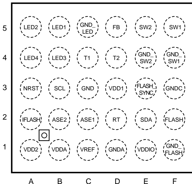
Figure 1. Top View
