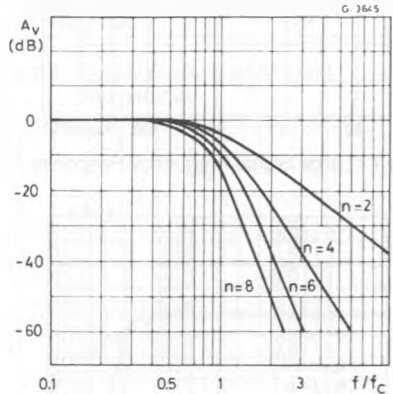
Figure 11 : Amplitude Response.
