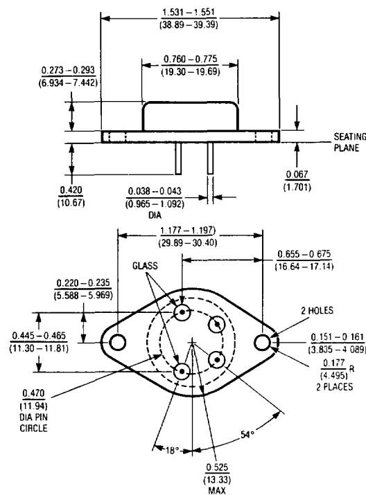
4-Pin Metal Package Similar to JEDEC T0-3
