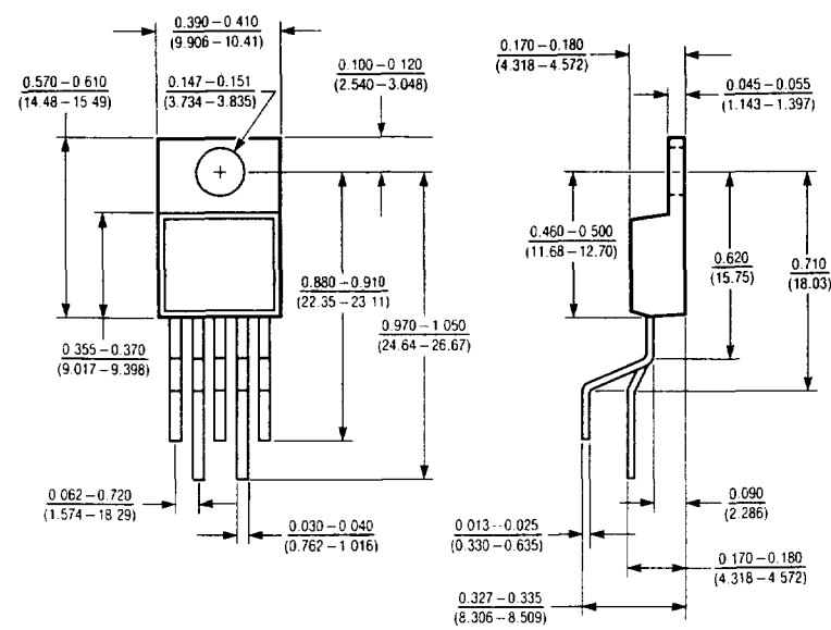
T0-220 Package (5 Lead)
