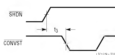
\overline{SHDN} to \overline{CONVST} Wake-Up Timing
