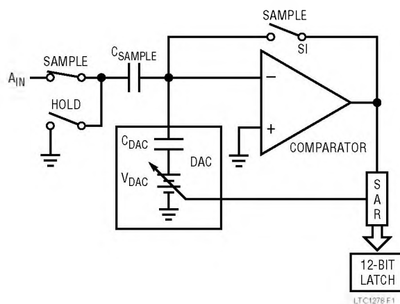
Figure 1. A_{IN} Input
