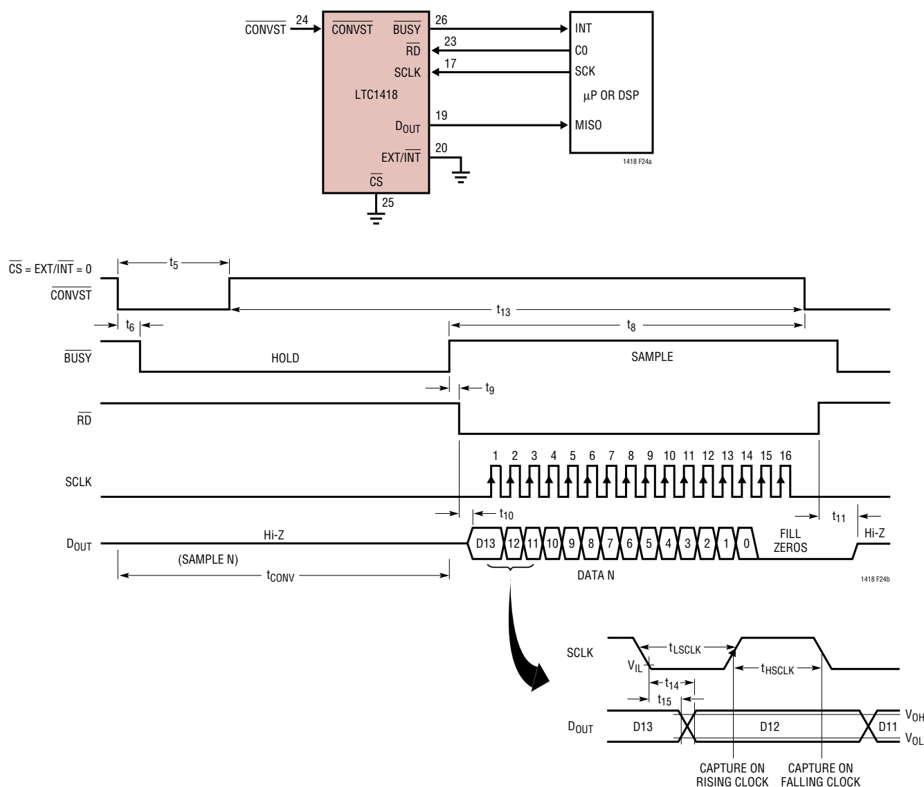
Figure 24. Internal Conversion Clock Selected. Data Transferred After Conversion Using an External SCLK. \overline{BUSY} ↑ Indicates End of Conversion
