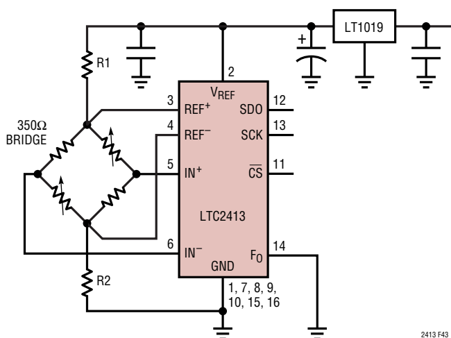
Figure 43. Simple Bridge Connection
