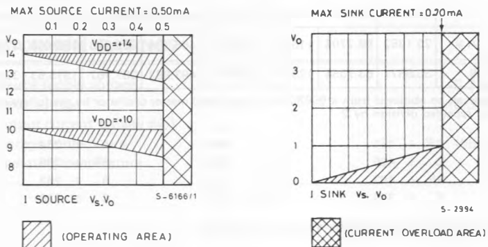
Fig. 2 - Output signal d.c. loading
