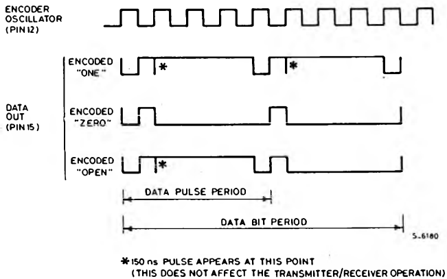
Figure 6 - Encoder Data Waveforms (M145026)
