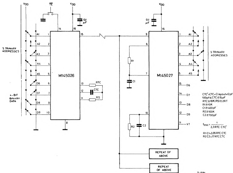
Example R/C Values (All Resistors and Capacitors are ± 5%) (CTC' = CTC + 20 pF)
