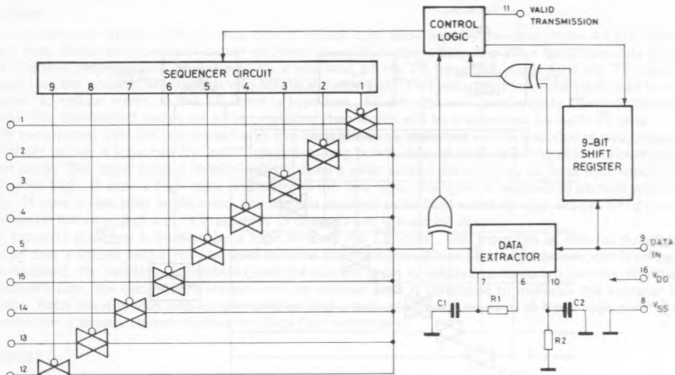
Fig. 3 – Decoder block diagram M145028
