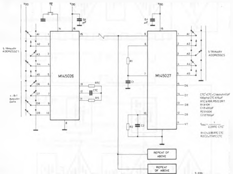
Figure 10 - Typical Application
