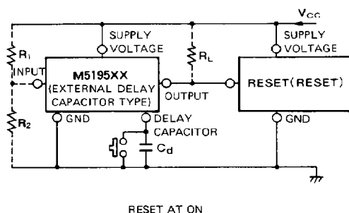
(a) Reset at ON
