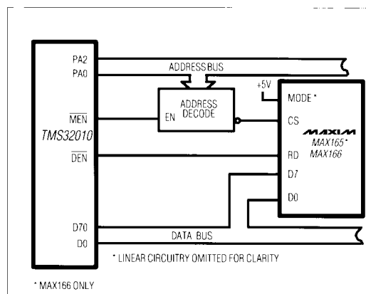
Figure 8. MAX165/MAX166 to TMS32010 ROM Interface
