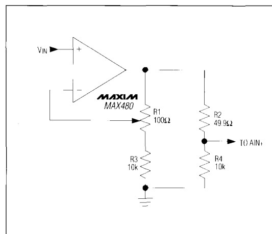
Figure 21a. Trim Circuit for Gain ( \pm 0.5\% )
