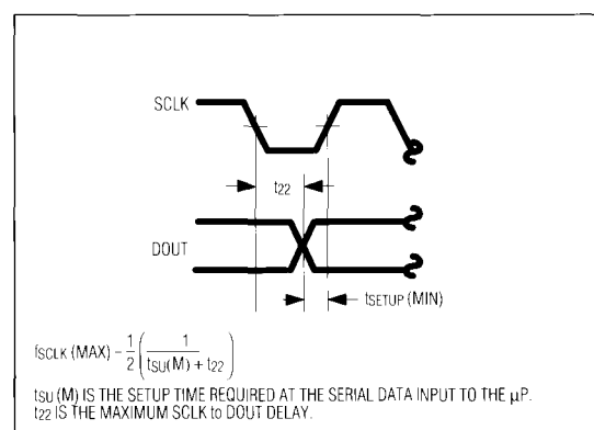
Figure 12. f_{SCLK}(MAX) is limited by the setup time required by the serial data input to the \mu P.
