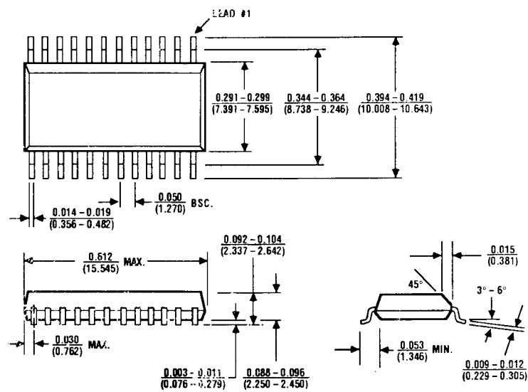
24 Lead Small Outline, Wide
