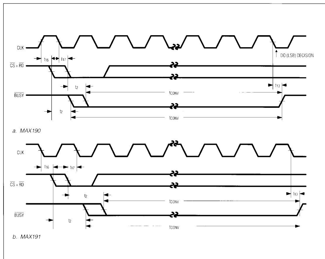
Figure 6. \overline{\text{CS}} , \overline{\text{RD}} , and CLK Synchronous Operation
