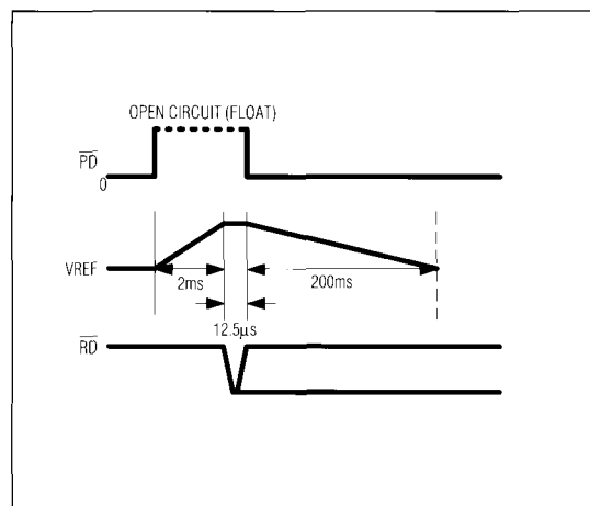
Figure 19b. Low Average-Power Mode Operation (External Compensation)
