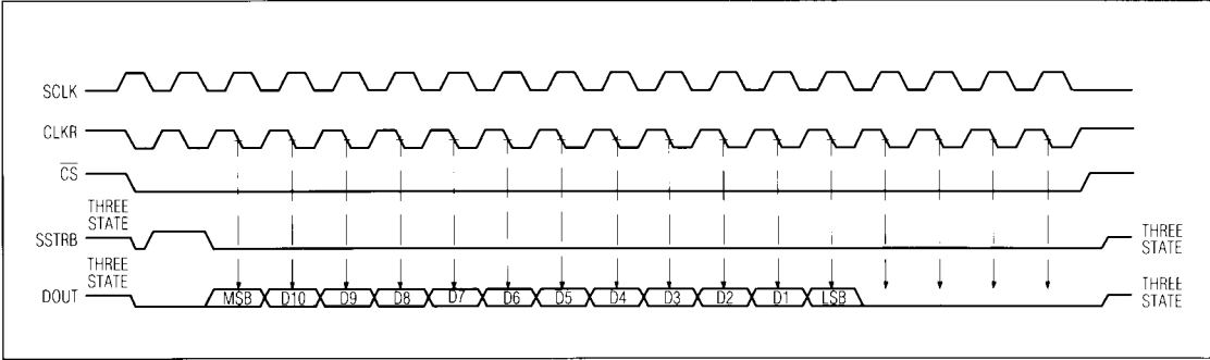
Figure 16. MAX190/MAX191 TMS320C4x Interface Timing
