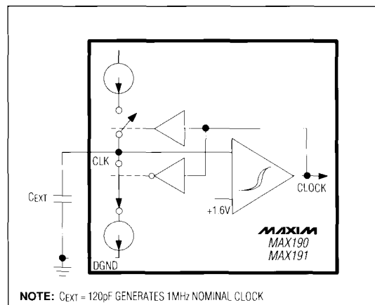
Figure 5. Internal Clock Circuit
