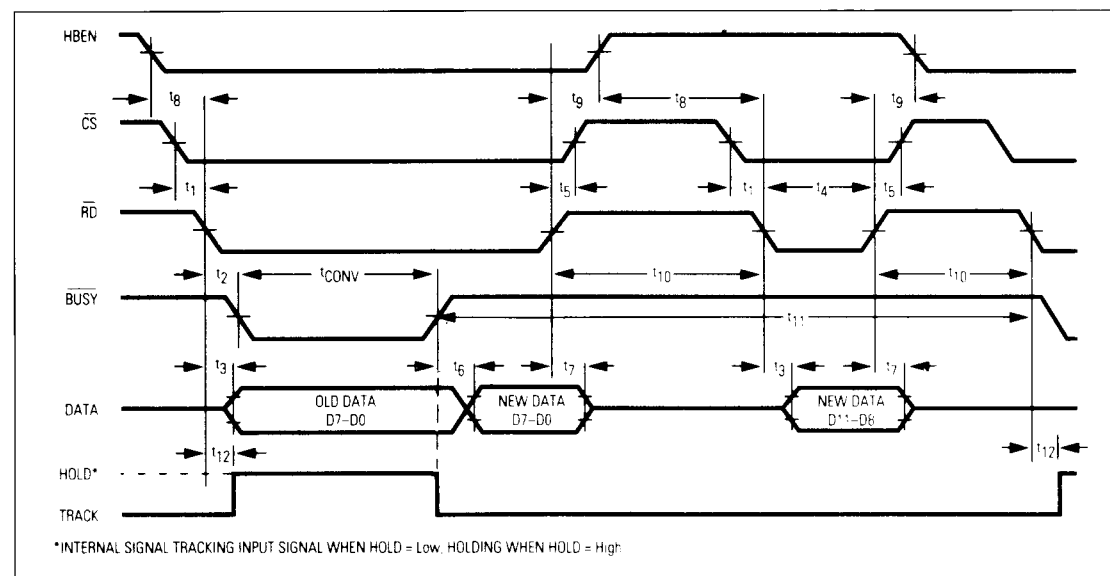
Figure 7. Slow-Memory Mode, 2-Byte Read Data-Bus Status
