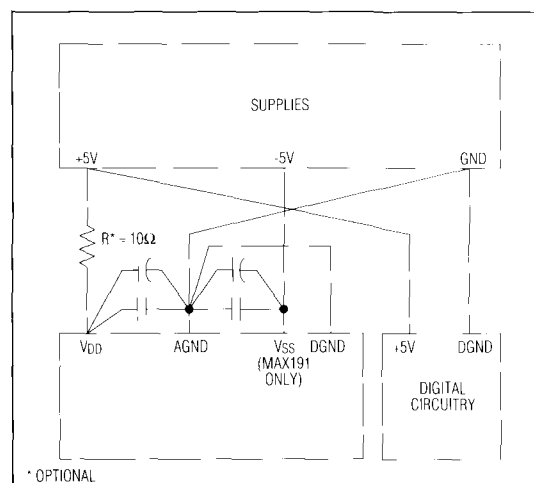
Figure 23. Power-Supply Grounding Connection
