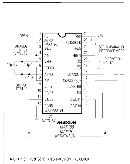
Figure 3. MAX190/MAX191 Operational Diagram
