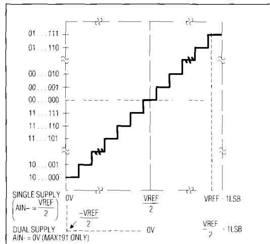
Figure 22. MAX190/MAX191 Bipolar Transfer Function
