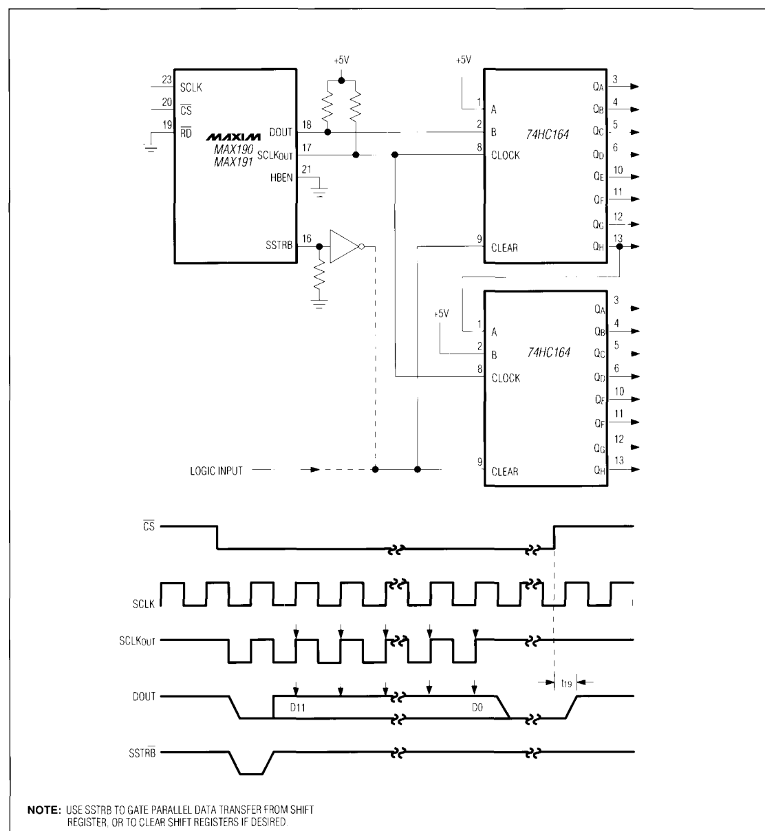
Figure 11. Simple Serial-to-Parallel Interface
