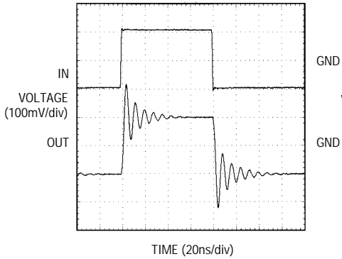
SMALL-SIGNAL PULSE RESPONSE ( A_{vCL} = +1V/V , C_L = 100pF )
