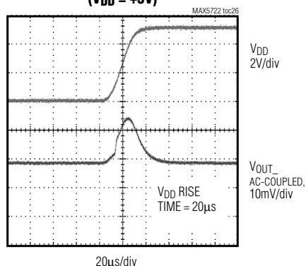
POWER-ON RESET, FAST RISE TIME ( V_{DD} = +3\text{V} )
