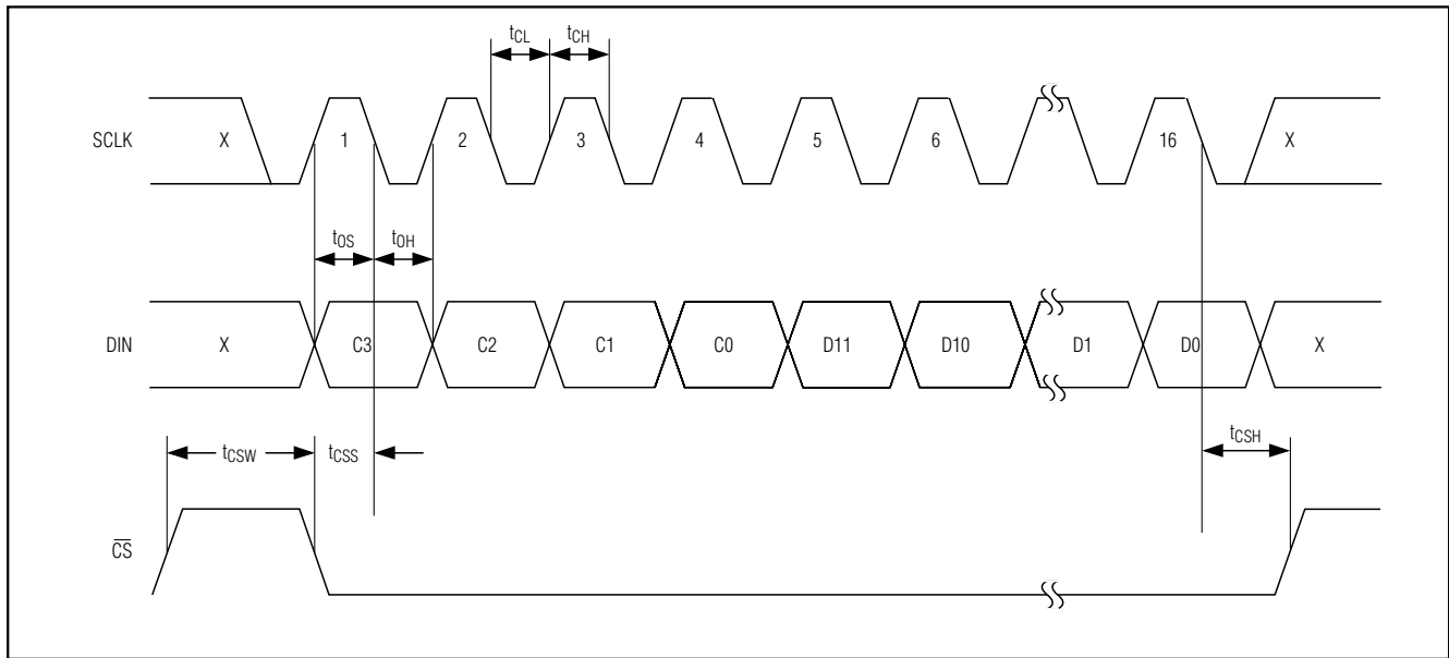
Figure 2. Timing Diagram
