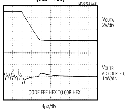
CROSSTALK ( V_{DD} = +5\text{V} )
