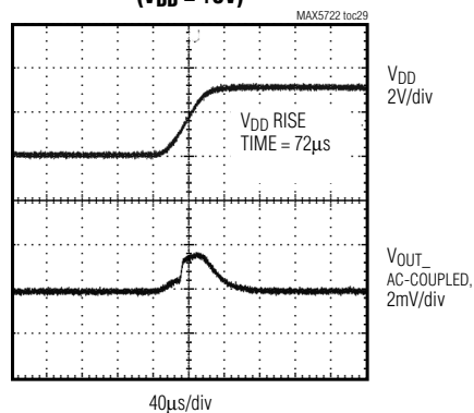
POWER-ON RESET, SLOW RISE TIME ( V_{DD} = +3\text{V} )
