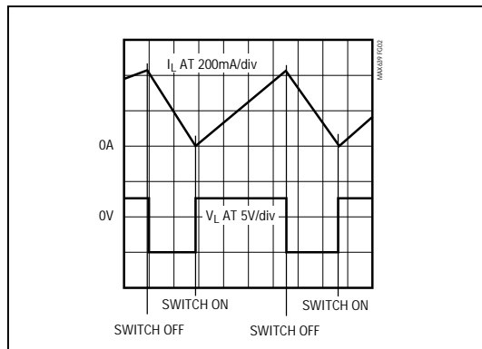
Figure 2. Simplified Step-Down Converter Operation
