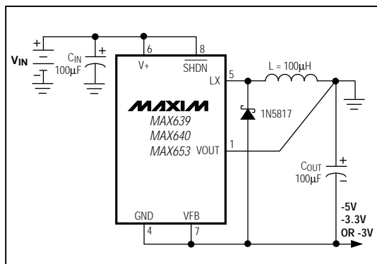
Figure 6. Inverting Configuration
