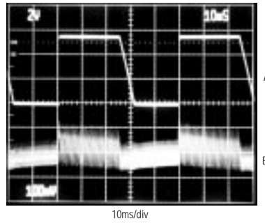
MAX639 LINE-TRANSIENT RESPONSE
