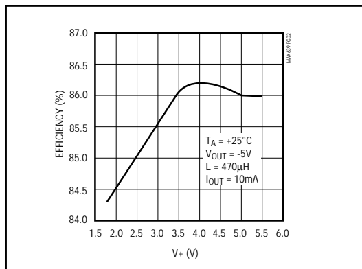
Figure 8. Efficiency of Figure 6 Circuit
