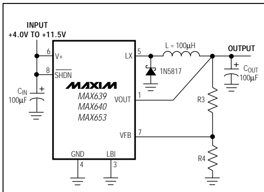
Figure 4. Adjustable-Output Operation
