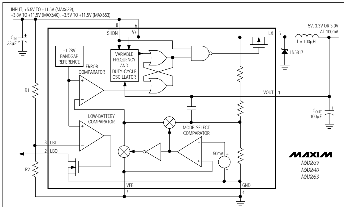
Figure 3. Block Diagram
