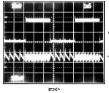
MAX639 LOAD-TRANSIENT RESPONSE
