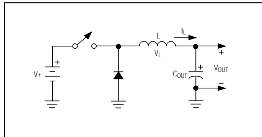
Figure 1. Simplified Step-Down Converter
