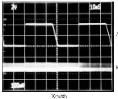
MAX653 LINE-TRANSIENT RESPONSE
