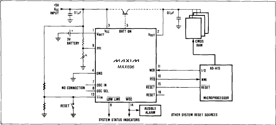
Figure 1. MAX696 Typical Application
