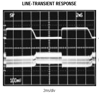
CIRCUIT OF FIGURE 2 V_{OUT} = -5\text{V} , I_{LOAD} = 1\text{A} A: V_+ , 3V TO 8V, 5V/div B: V_{OUT} , 100mV/div, AC-COUPLED
