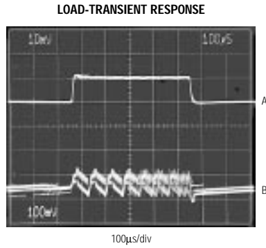
CIRCUIT OF FIGURE 2 V_+ = 6\text{V} , V_{OUT} = -5\text{V} A: I_{LOAD} , 30mA TO 1A, 1A/div B: V_{OUT} , 100mV/div, AC-COUPLED
