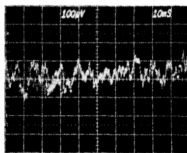
MAX874 1Hz TO 100Hz NOISE
