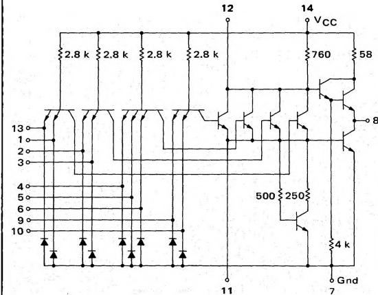
CIRCUIT SCHEMATIC
