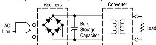
Figure 13. Uncorrected Power Factor Circuit
