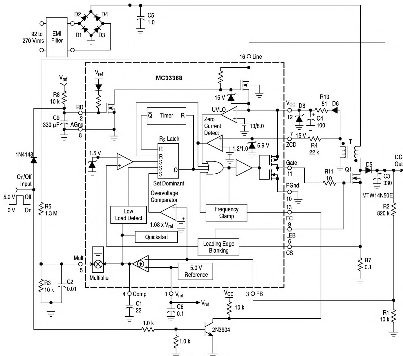
Figure 18. On/Off Control
