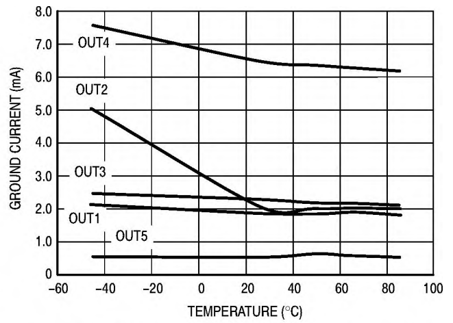
Figure 10. Ground Current versus Individual Output
