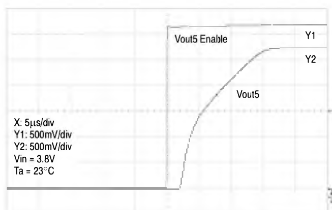
Figure 4. Output response from separate Enable
