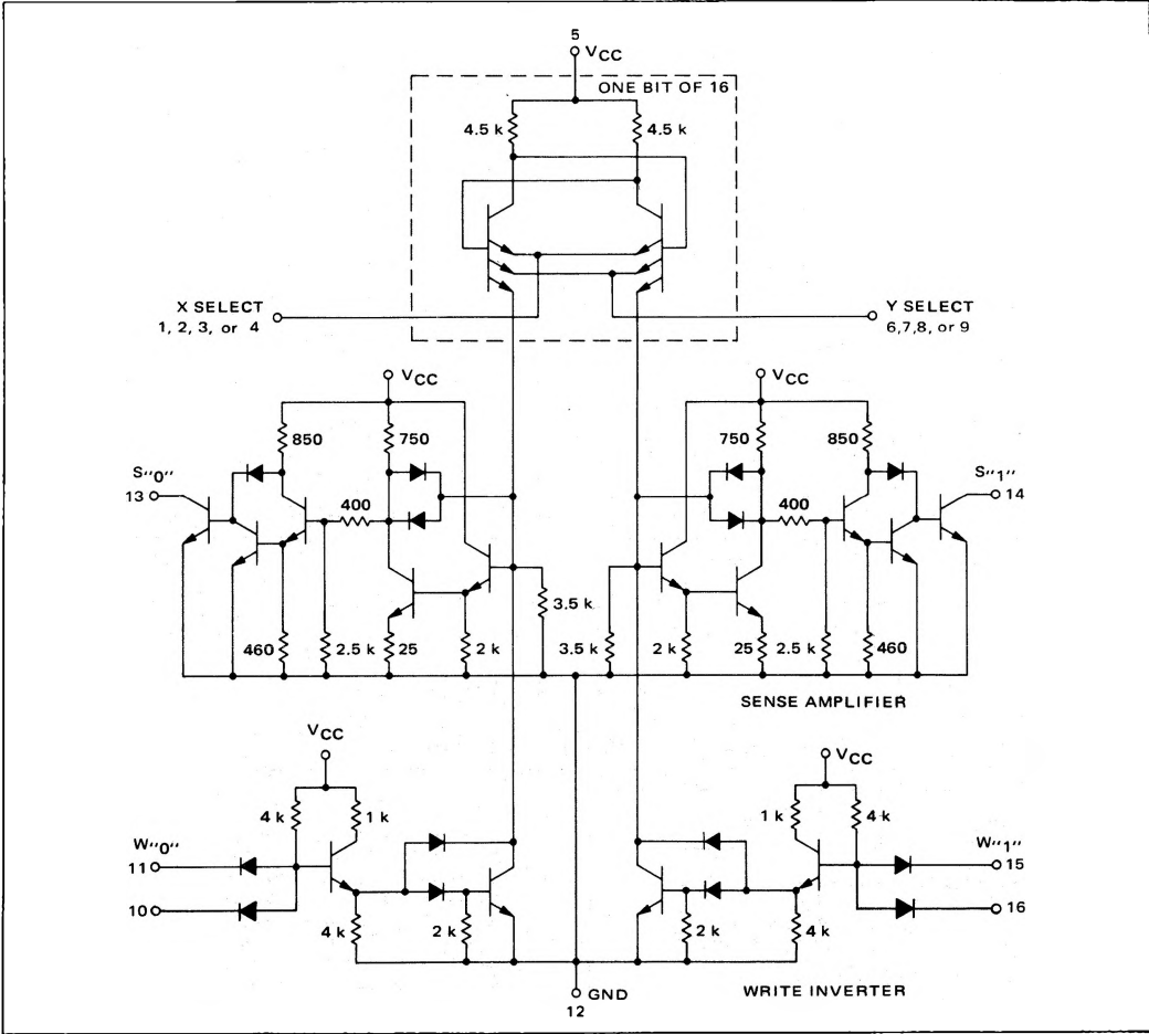
CIRCUIT SCHEMATIC
