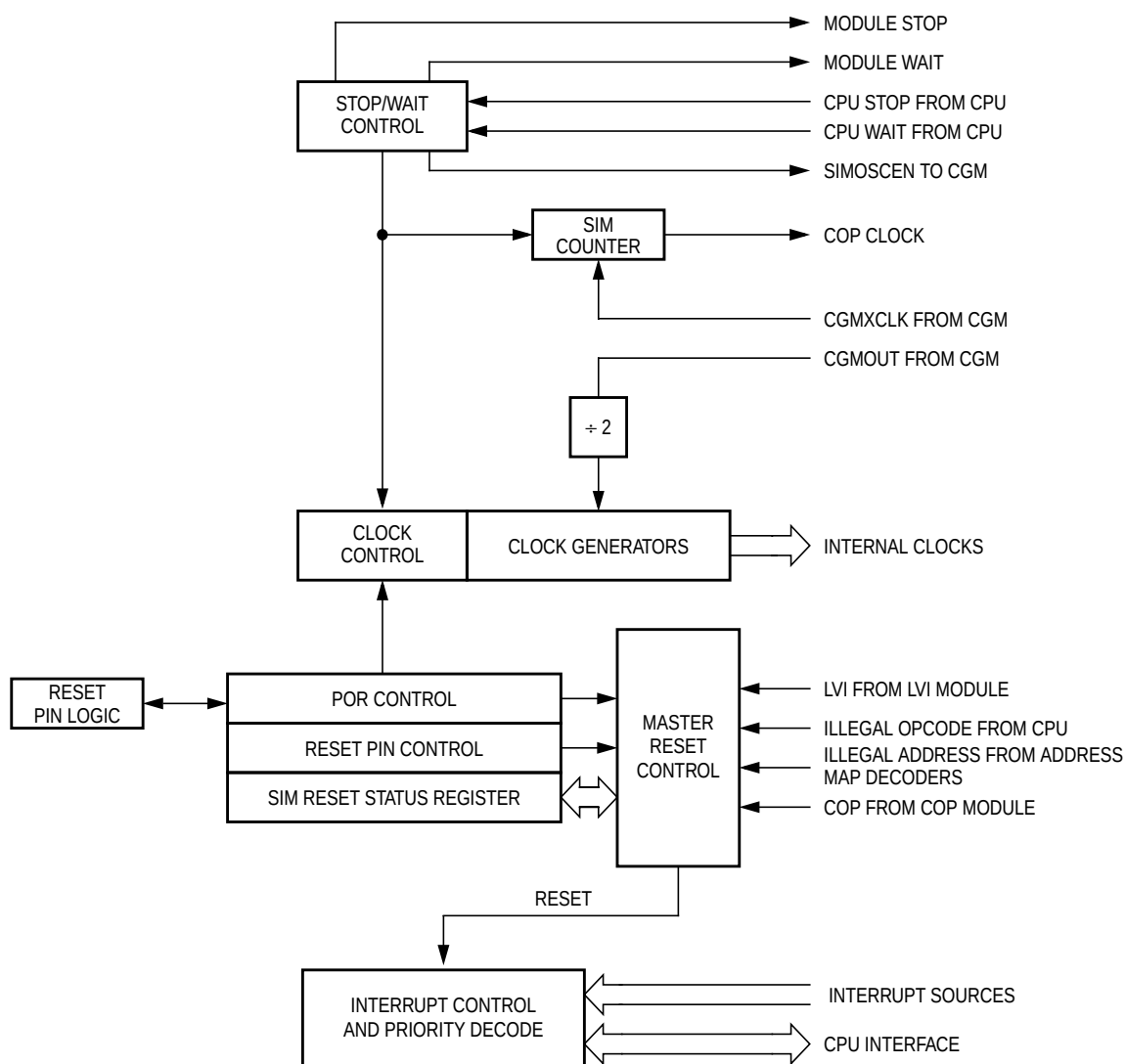
Figure 9-1. SIM Block Diagram
