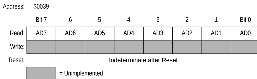
Figure 19-3. ADC Data Register (ADR)
