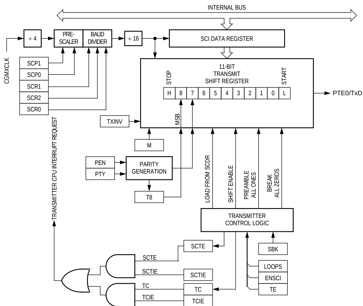
Figure 17-3. SCI Transmitter
