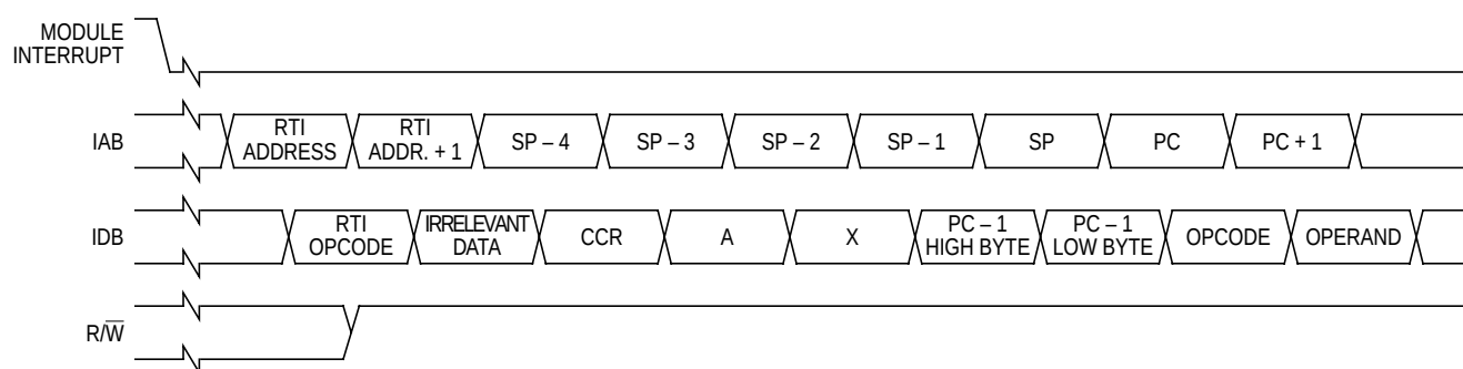
Figure 9-9. Hardware Interrupt Recovery Timing
