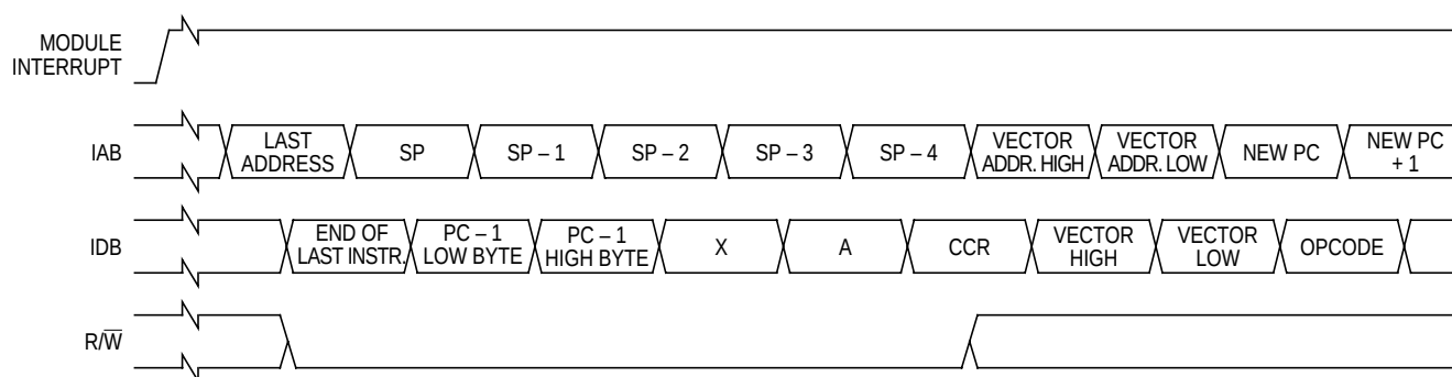
Figure 9-7. Hardware Interrupt Entry Timing
