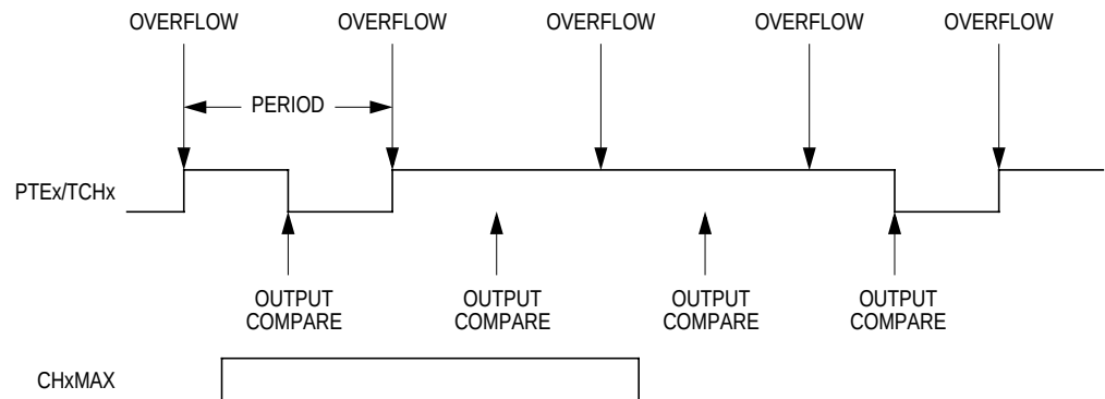
Figure 16-7. CHxMAX Latency
