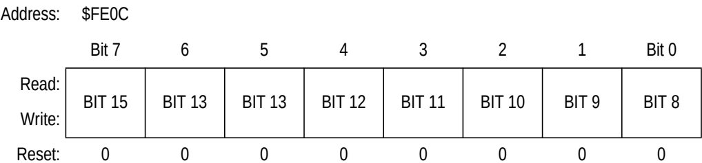
Figure 11-3. Break Address Register (BRKH)
