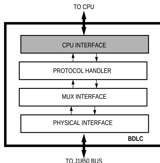
Figure 20-14. BDLC Block Diagram
