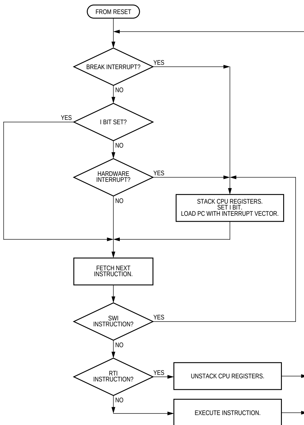
Figure 9-8. Interrupt Processing
