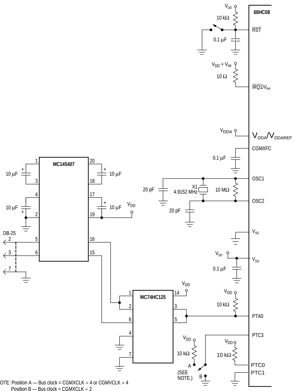
Figure 12-1. Monitor Mode Circuit
