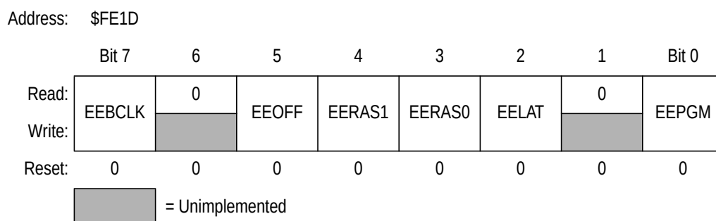
Figure 6-1. EEPROM Control Register (EECR)
