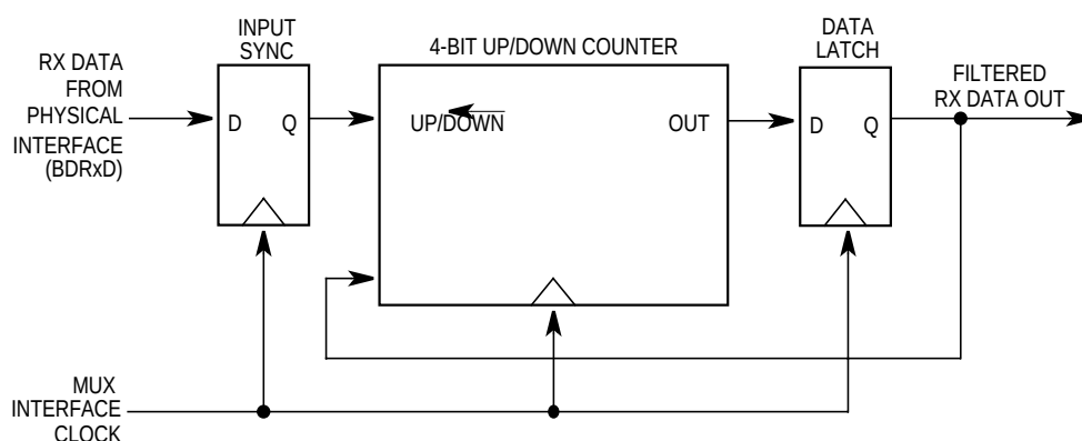
Figure 20-4. BDLC Rx Digital Filter Block Diagram
