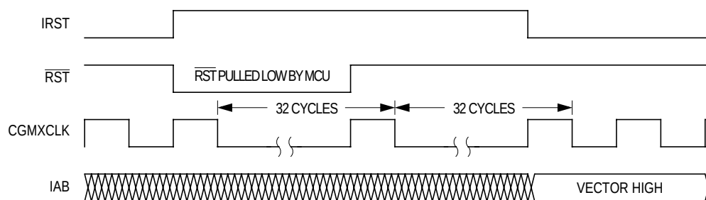
Figure 9-4. Internal Reset Timing
