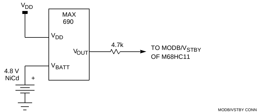
Figure 4-3 RAM Standby MODB/ V_{STBY} Connections
