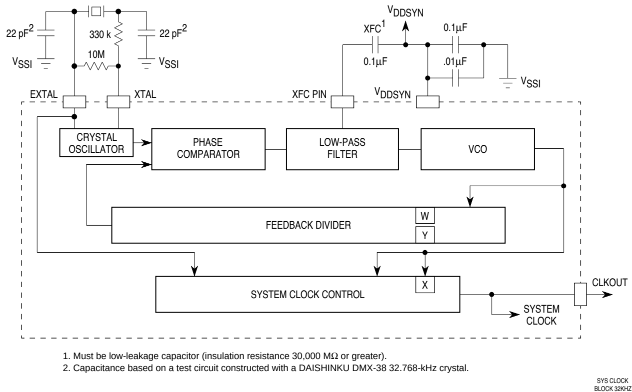
Figure 5 System Clock Block Diagram
