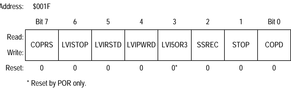
Figure 21-2. Configuration Register 1 (CONFIG1)
