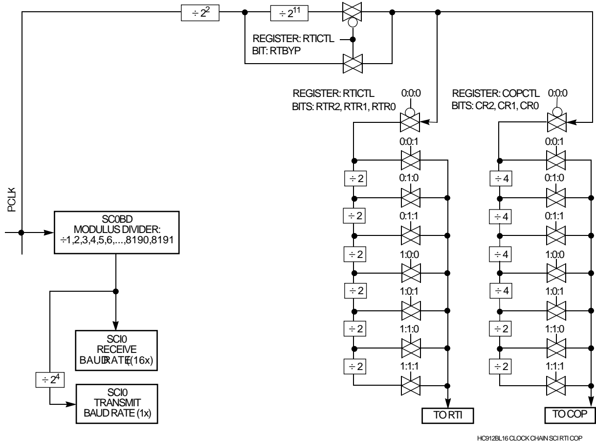
Figure 14 Clock Chain for SCI, RTI, COP
