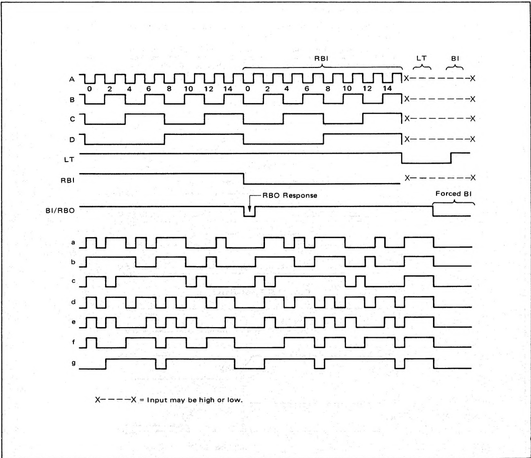
INPUT/OUTPUT VOLTAGE WAVEFORMS
