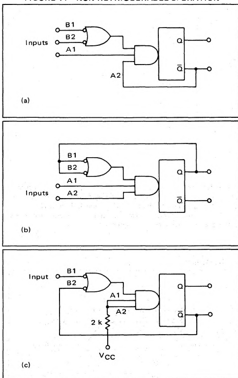
FIGURE 14 – NON-RETRIGGERABLE OPERATION
