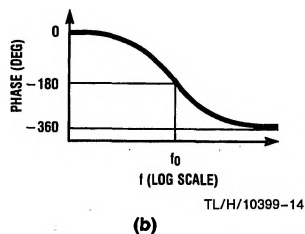
FIGURE 5. 2nd-Order All-Pass Response
