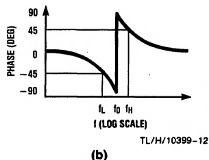
FIGURE 4. 2nd-Order Notch Response
