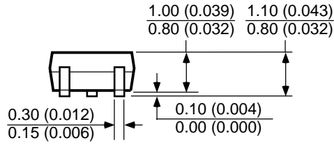
SC-70 (C5)
