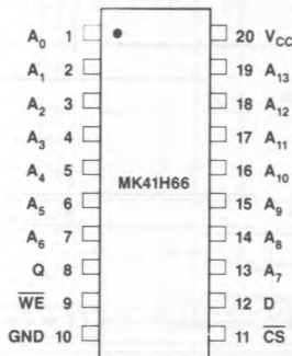
FIGURE 1. PIN CONNECTIONS
