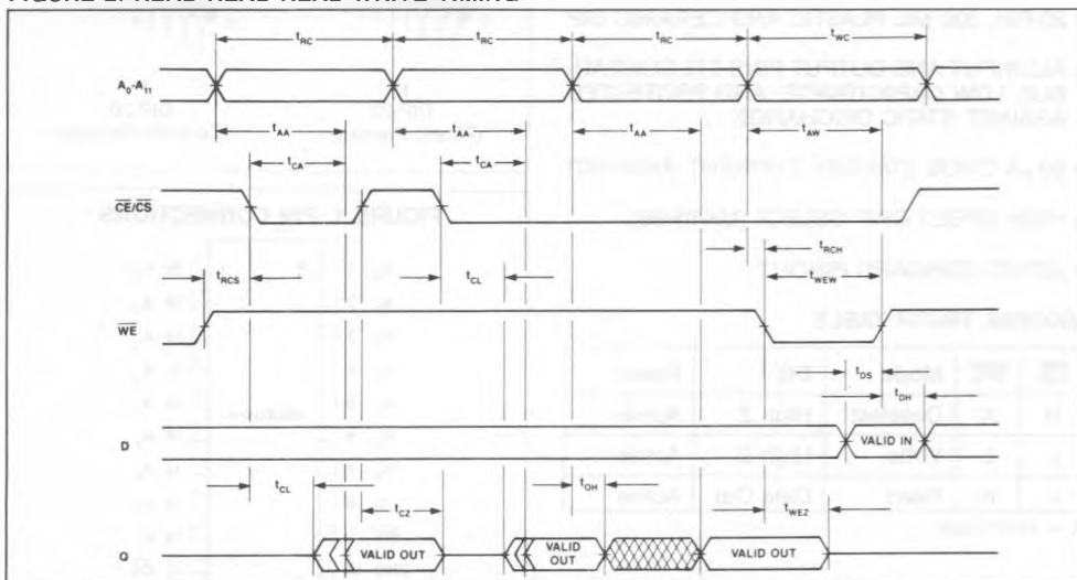
FIGURE 2. READ-READ-READ-WRITE TIMING
