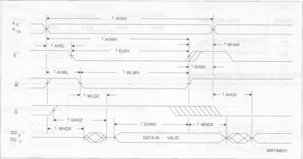
FIGURE 5 : CHIP ENABLE CONTROL WRITE CYCLE TIMING
