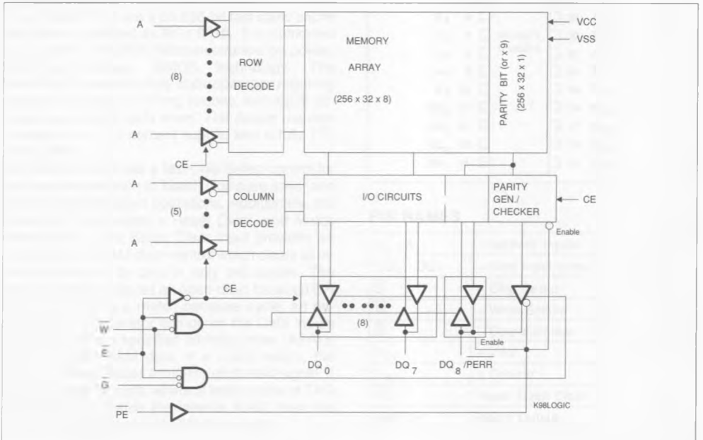
BLOCK DIAGRAM N o . 2
