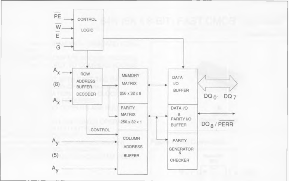
MK48H98/99 BLOCK DIAGRAM N o . 1
