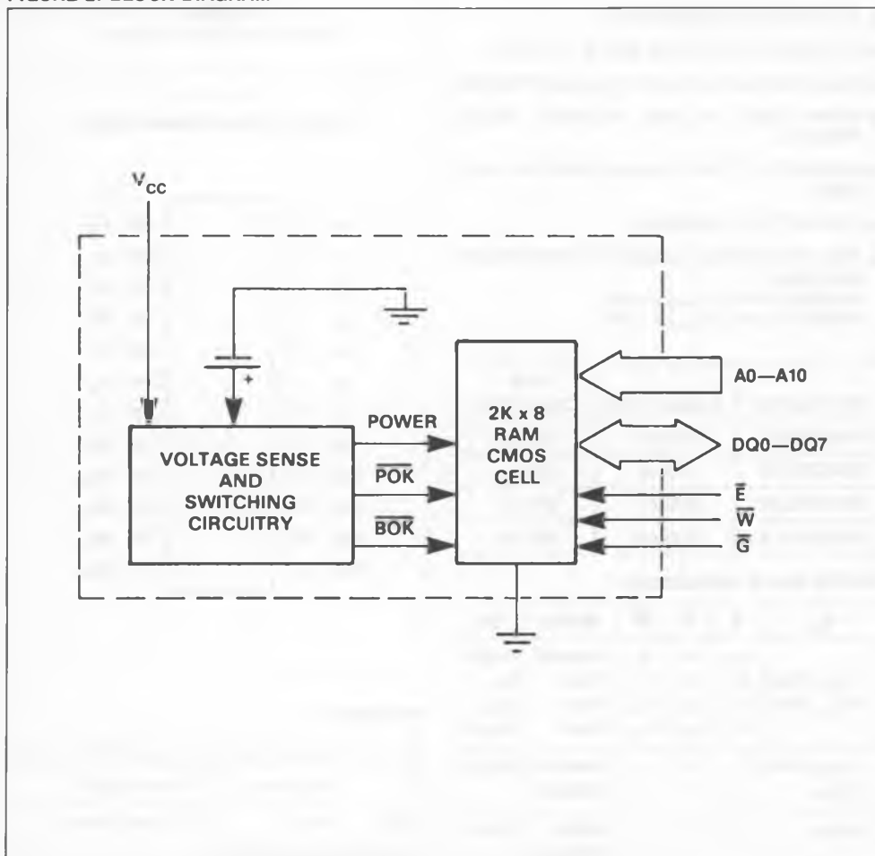
FIGURE 2. BLOCK DIAGRAM
