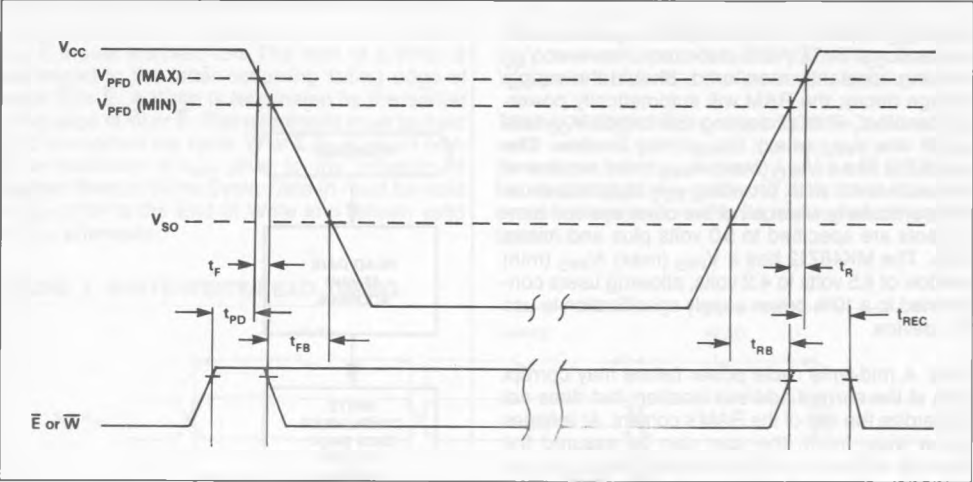
FIGURE 6. POWER-DOWN/POWER-UP TIMING
