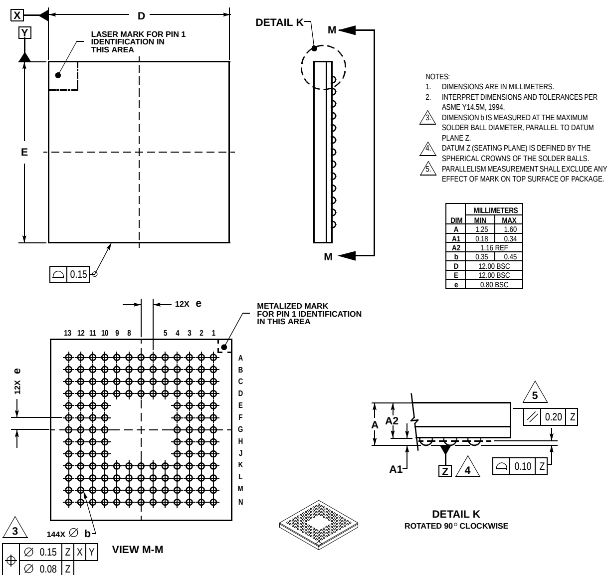
Figure 8. MMC2080/2075 BGA Mechanical Drawings
