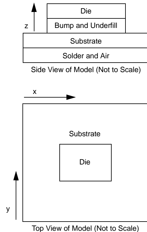
Figure 28. Recommended Thermal Model of MPC7447 and MPC7457
