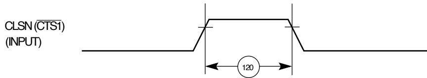
Figure 49. Ethernet Collision Timing Diagram
