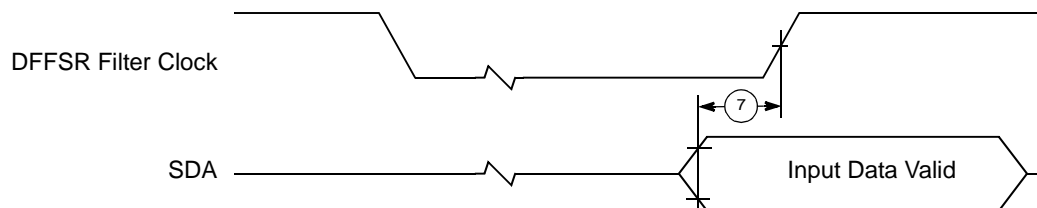
Figure 18. I²C Timing Diagram III
