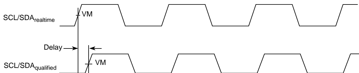
Figure 18. I²C Timing Diagram III
