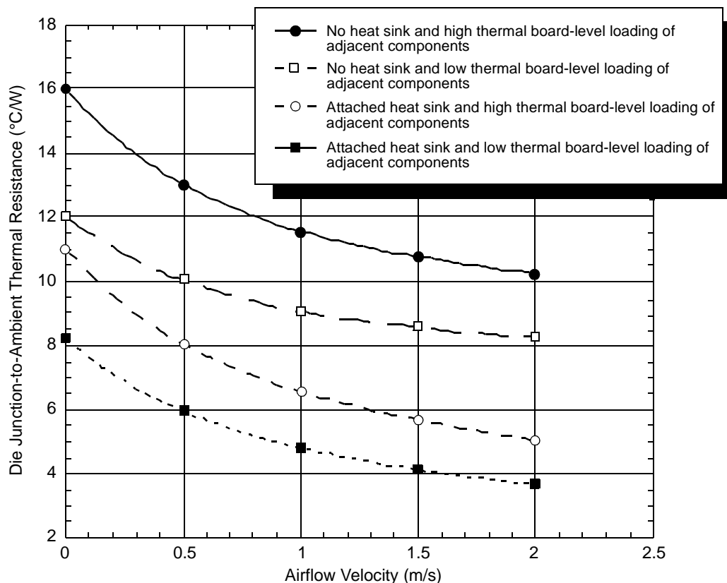
Figure 30. Die Junction-to-Ambient Resistance
