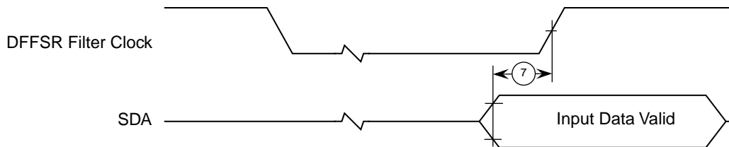
Figure 16. I²C Timing Diagram III
