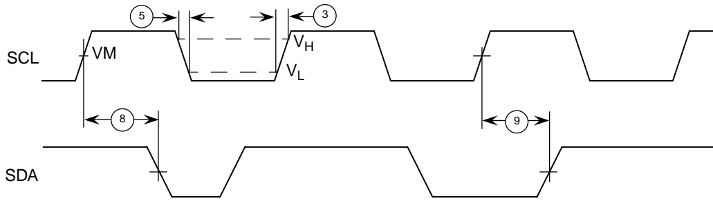
Figure 15. I²C Timing Diagram II
