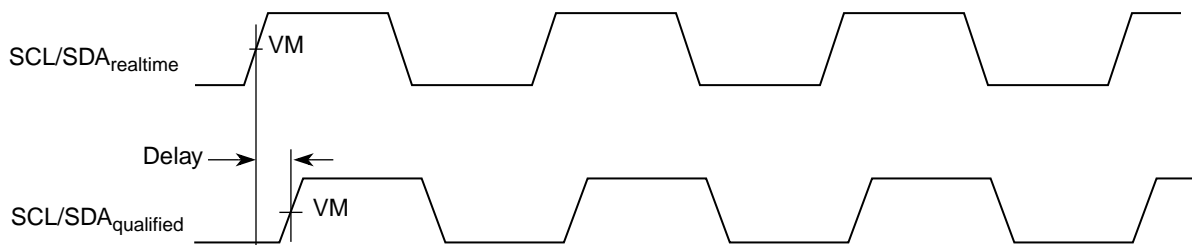
Figure 17. I²C Timing Diagram IV (Qualified Signal)
