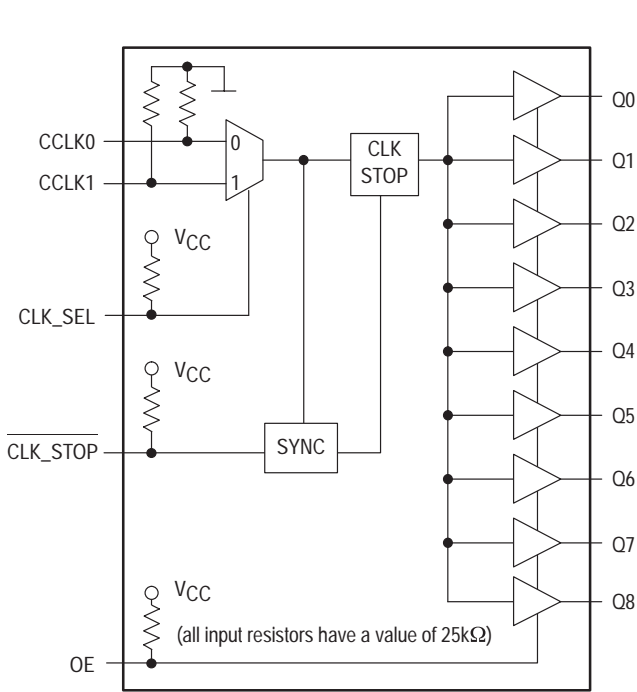
Figure 1. Logic Diagram
