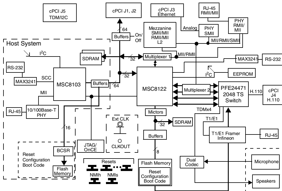
Figure 1. MSC8122ADS Block Diagram
