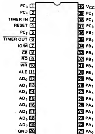
MSM81C55RS (Top View) MSM81C55-5RS 40 Load Plastic DIP
