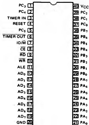
MSM81C55RS (Top View) MSM81C55-5RS 40 Lead Plastic DIP
