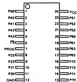
MSM82C43GS (Top View) 24 Lead Plastic Flat Package
