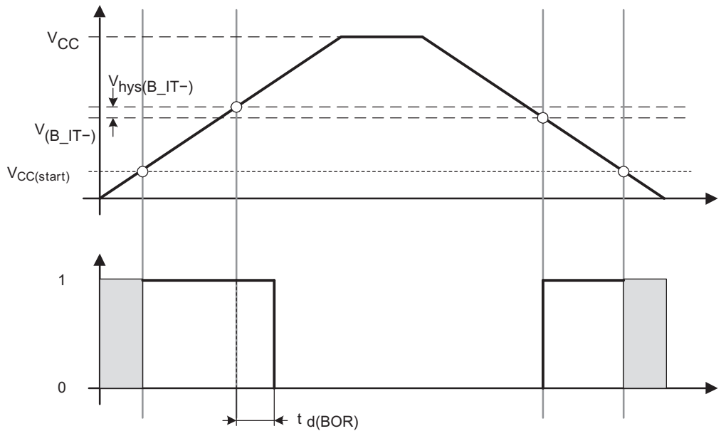
Figure 8. POR/Brownout Reset (BOR) vs Supply Voltage
