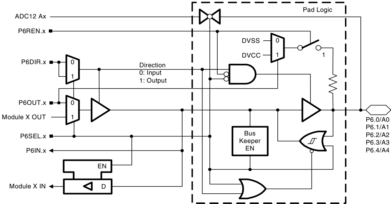
Port P6.0 to P6.4 pin functions
