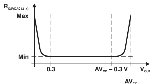
Figure 18. DAC12_x Output Resistance Tests
